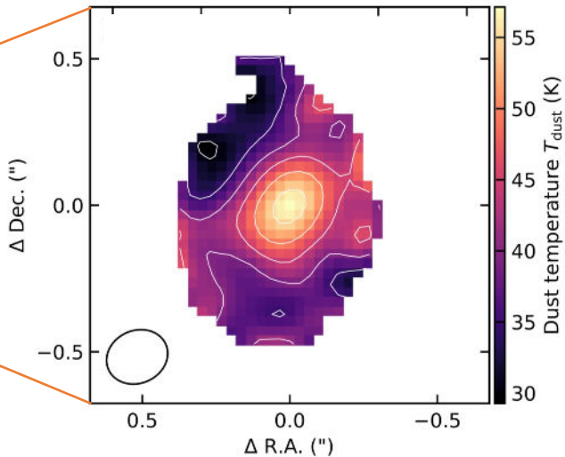
Dust temperature map
